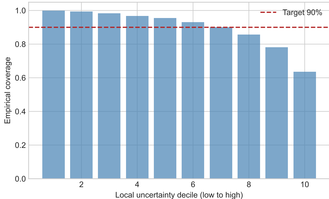
Coverage by local uncertainty level
