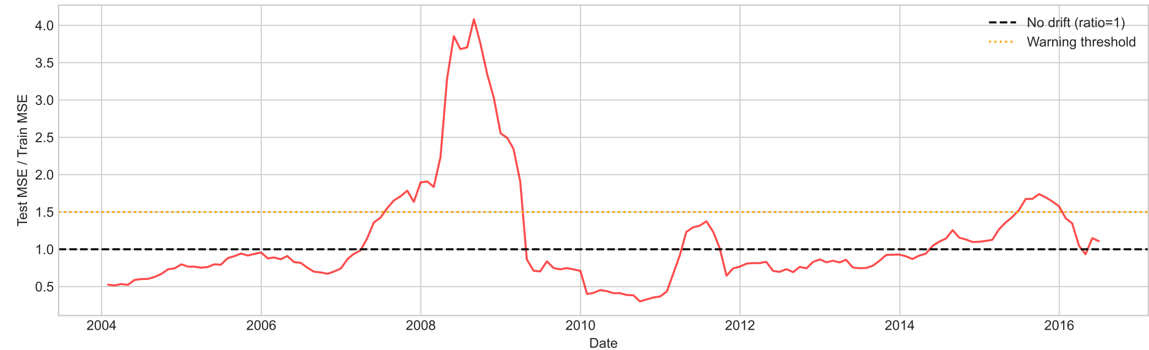
Drift Detection: Test/Train MSE Ratio
