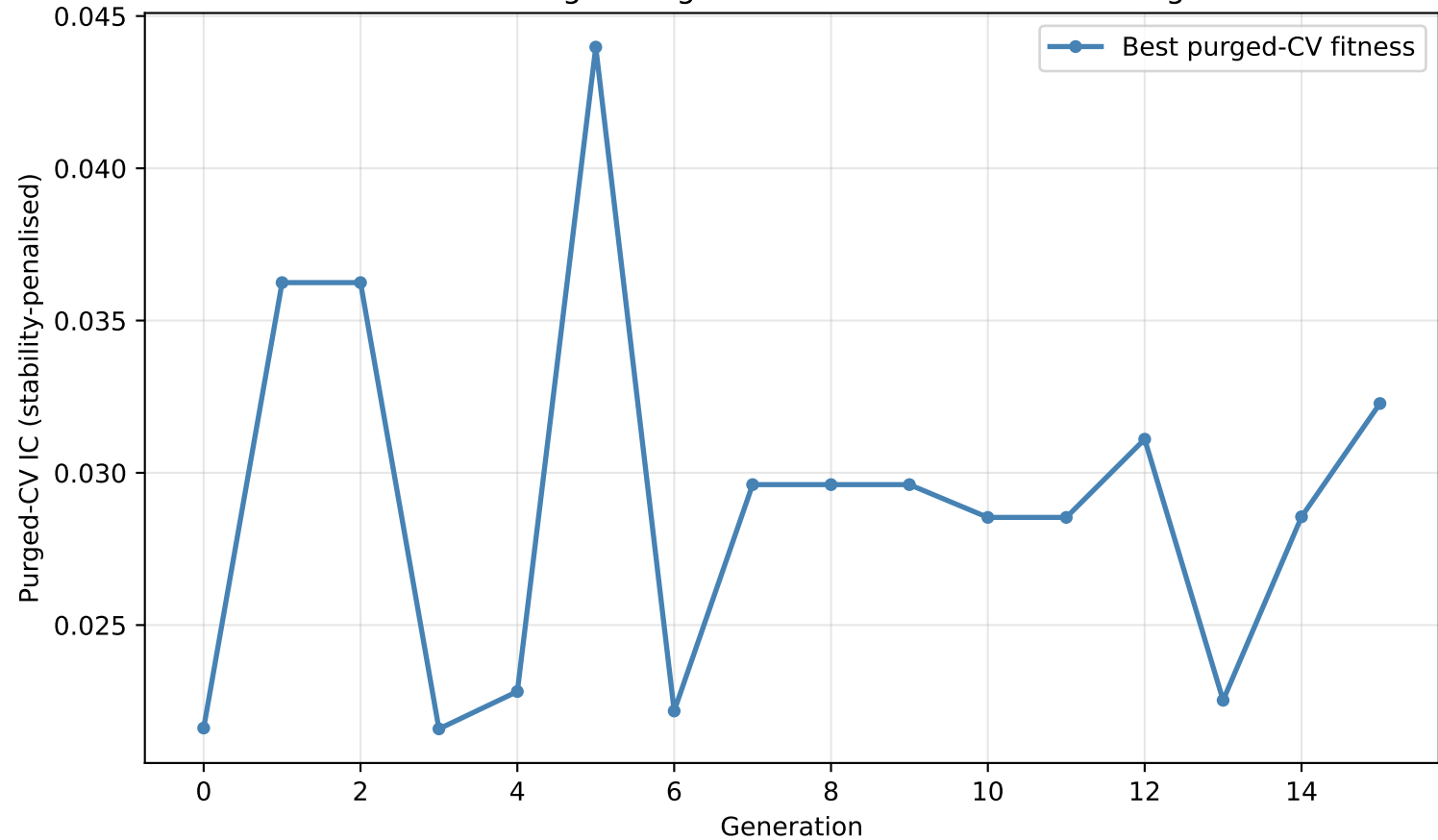
GA Convergence: generalization-aware GBR tuning
