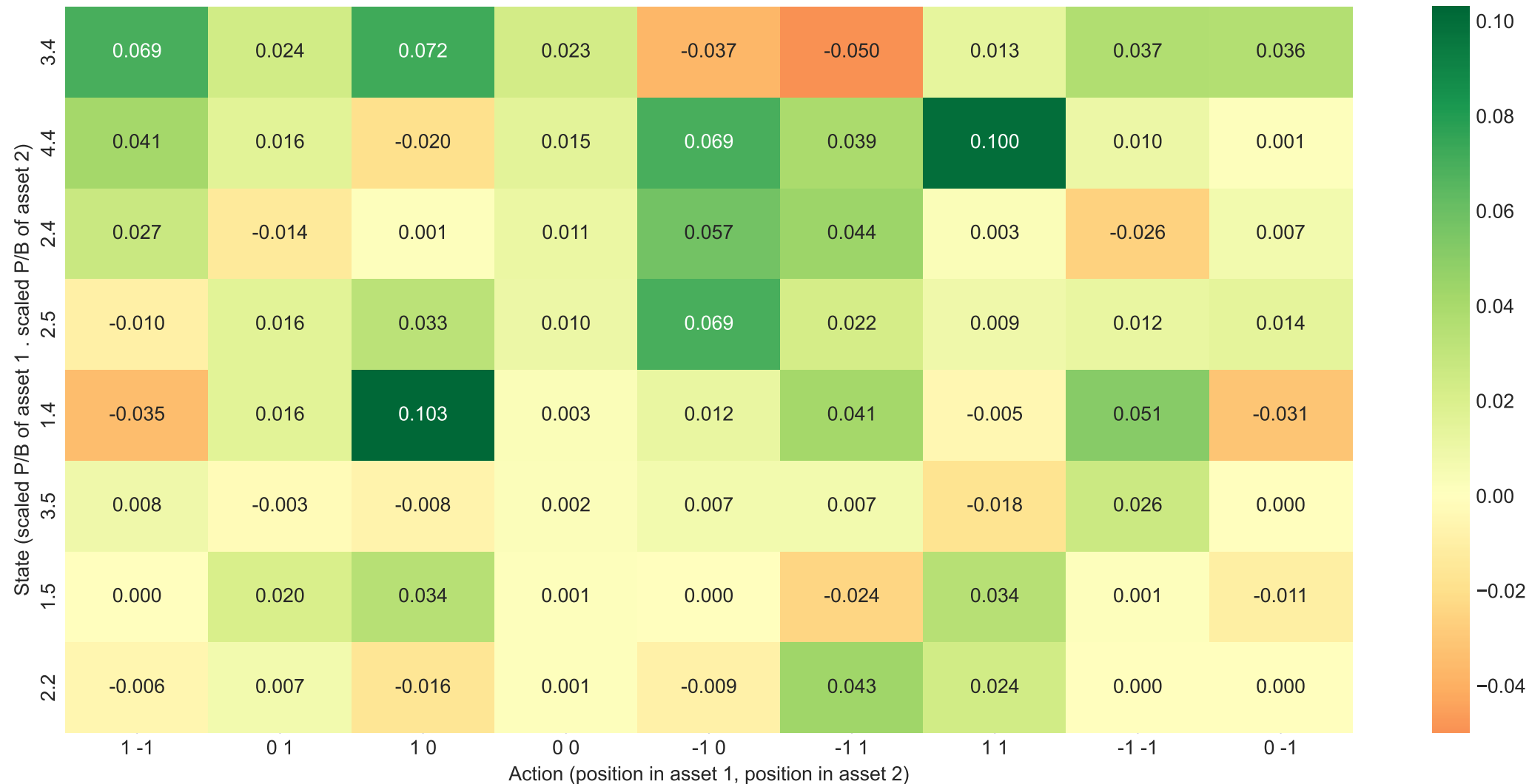
Q-values for Most Common States in Market Data
