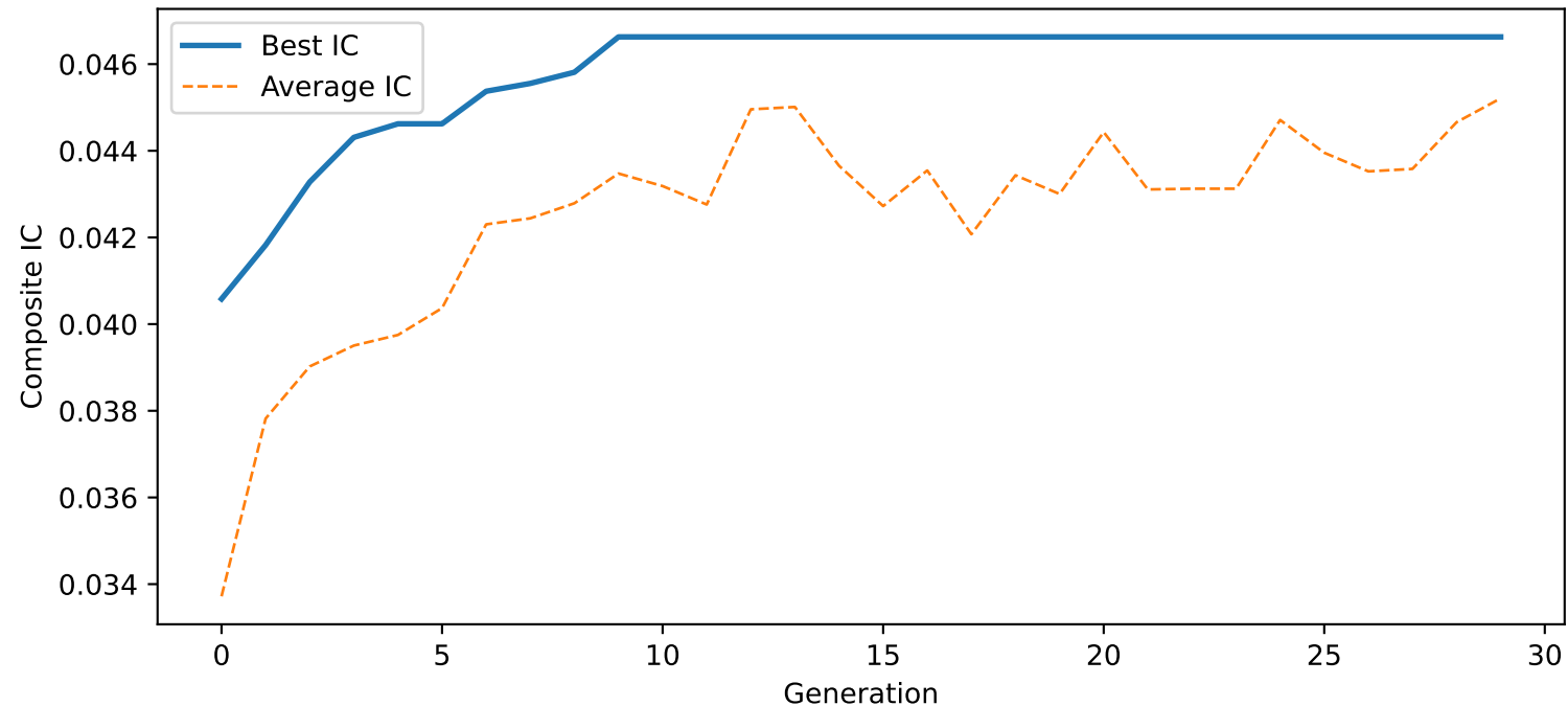
Miniature feature-selection GA: convergence
