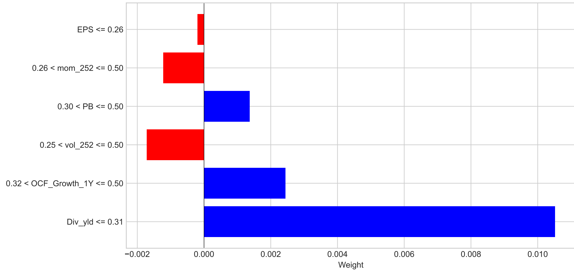
LIME Explanation for Instance 2
