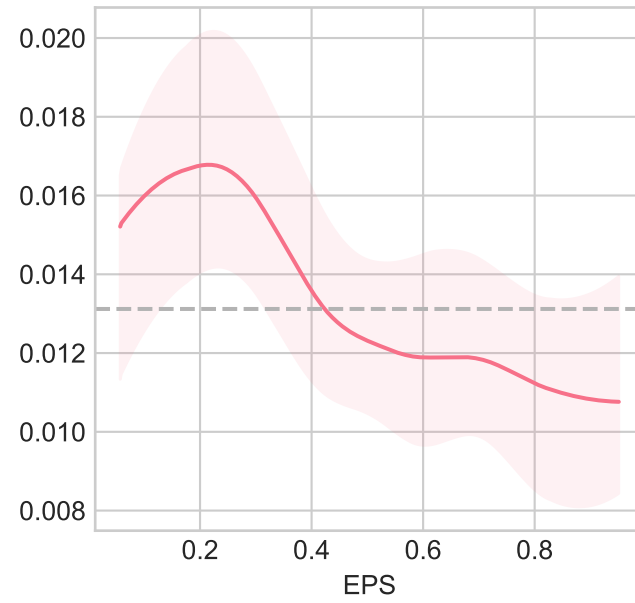
Partial Dependence Plots - BART Model
