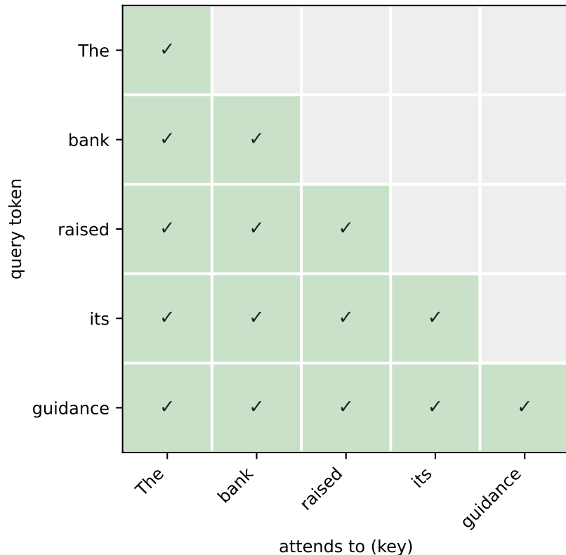
Decoder (GPT-style)
