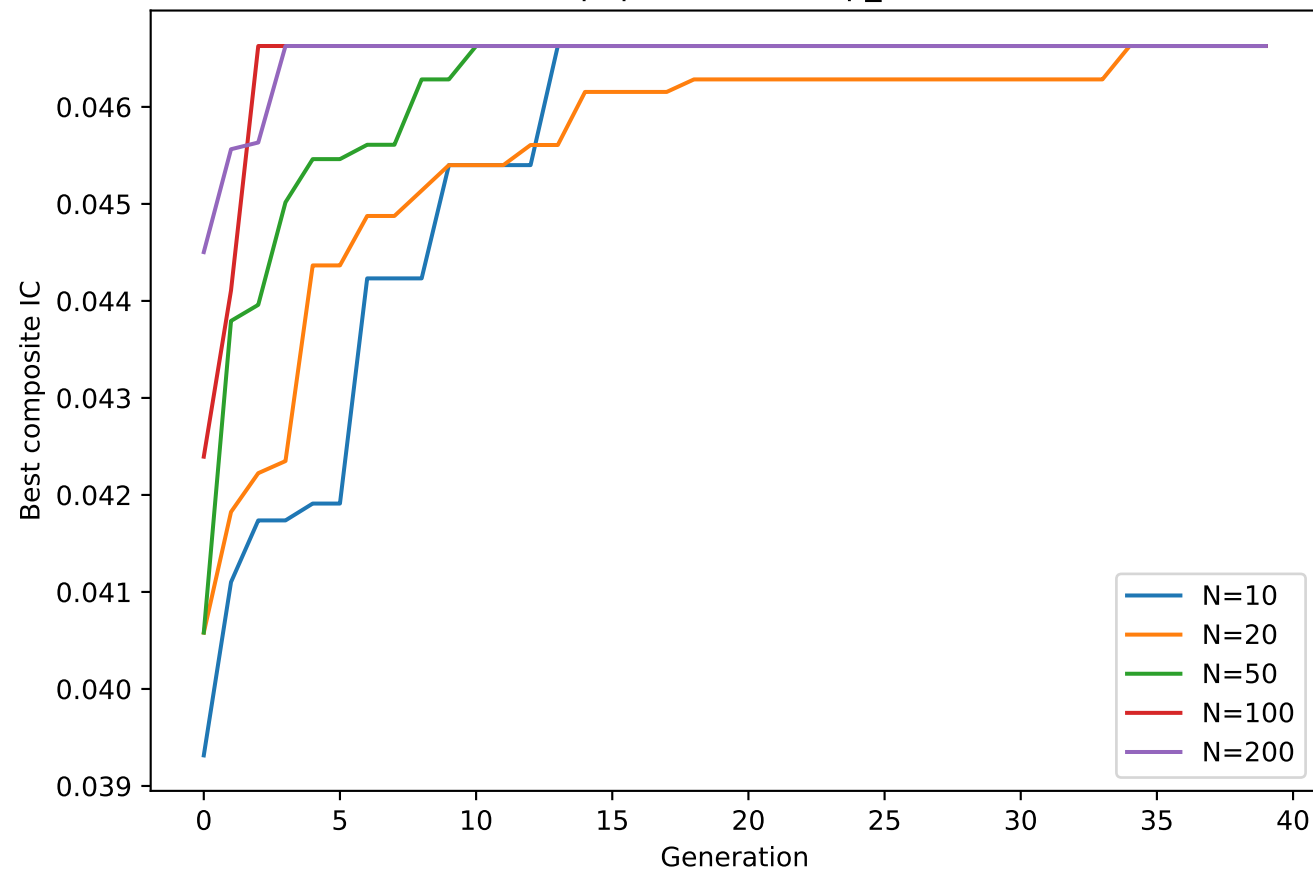
Effect of population size ( p_{mut}=1/L )
