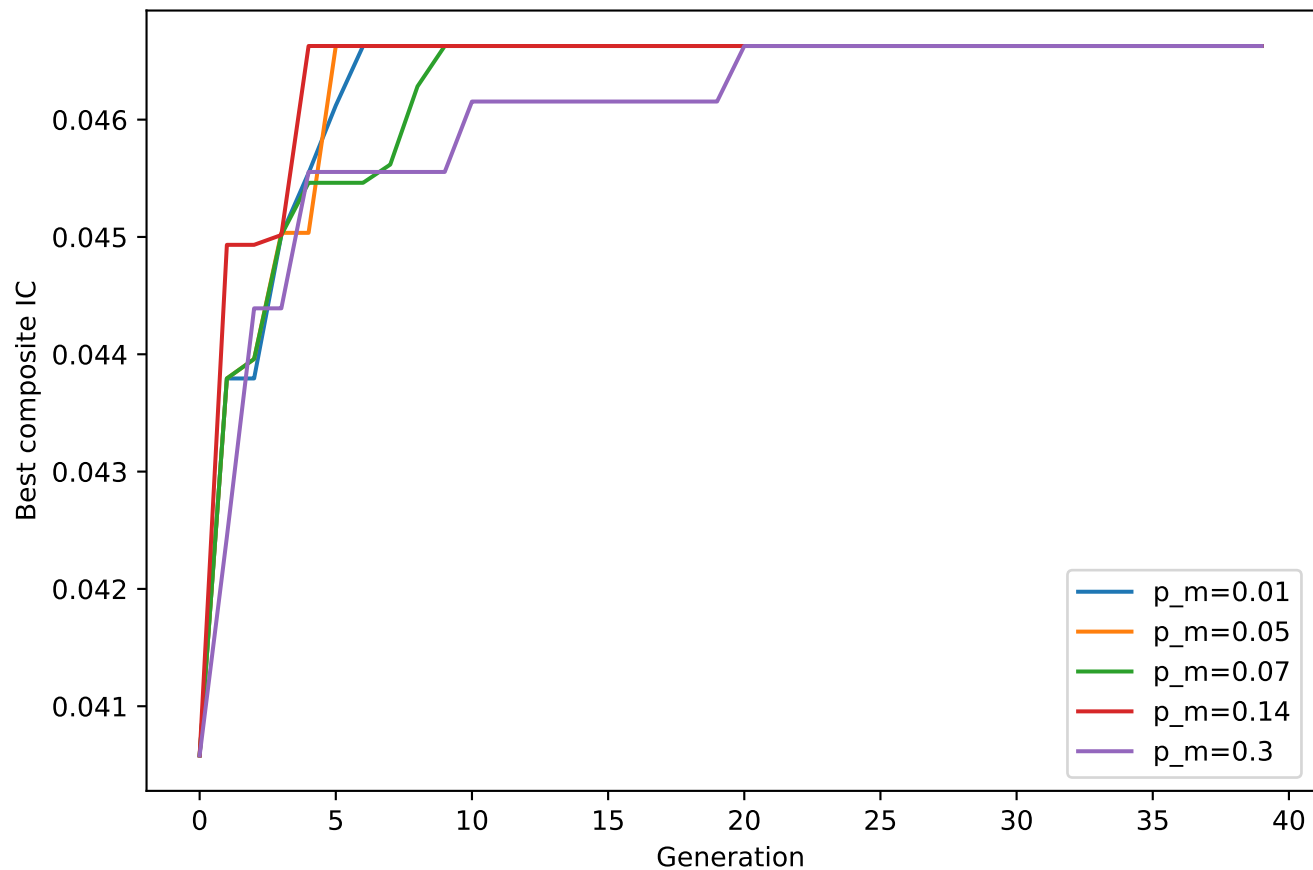
Effect of mutation rate ( N=50 )
