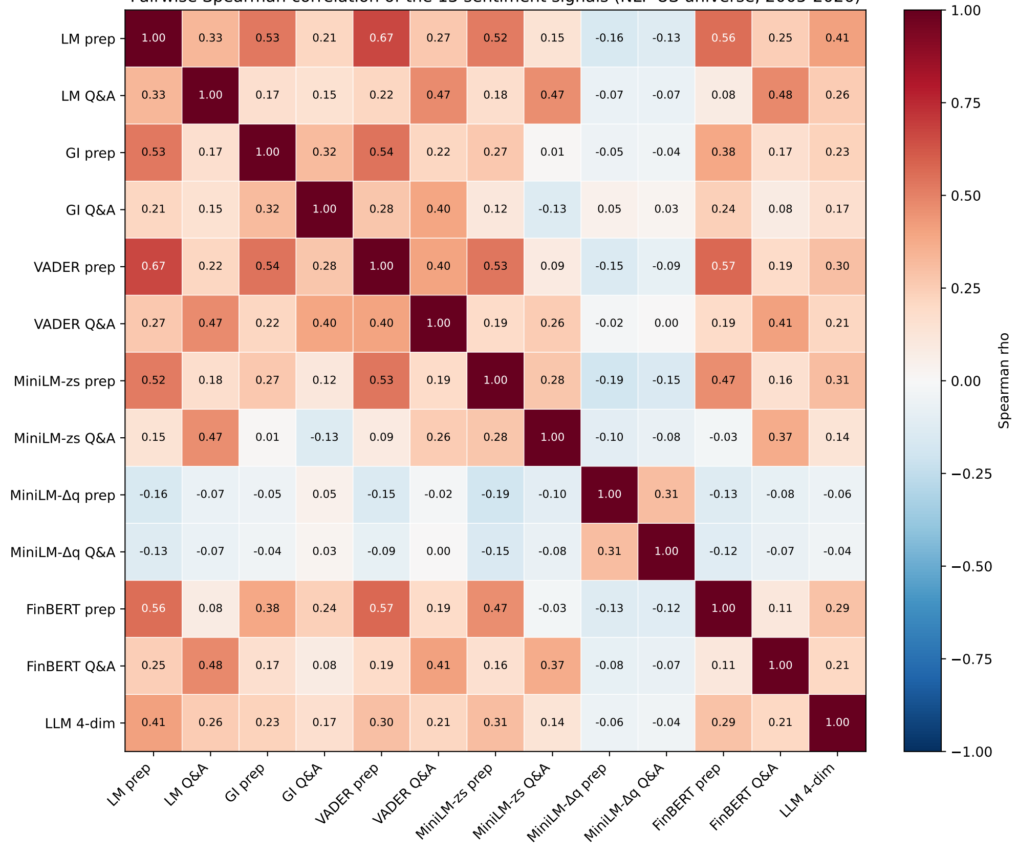
Pairwise Spearman correlation of the 13 sentiment signals (NLP US universe, 2005-2026)
