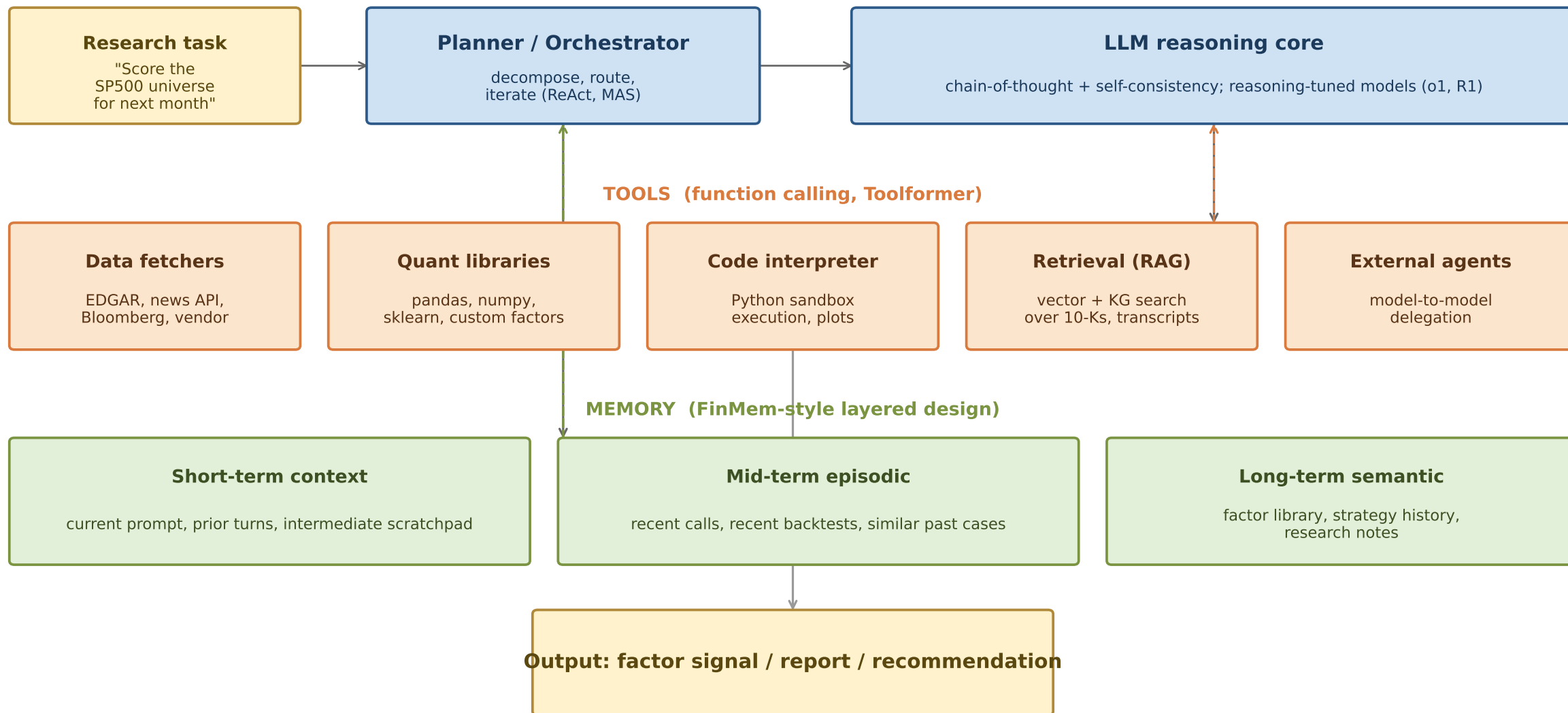
FIGURE 23.2: LLM-agent architecture
