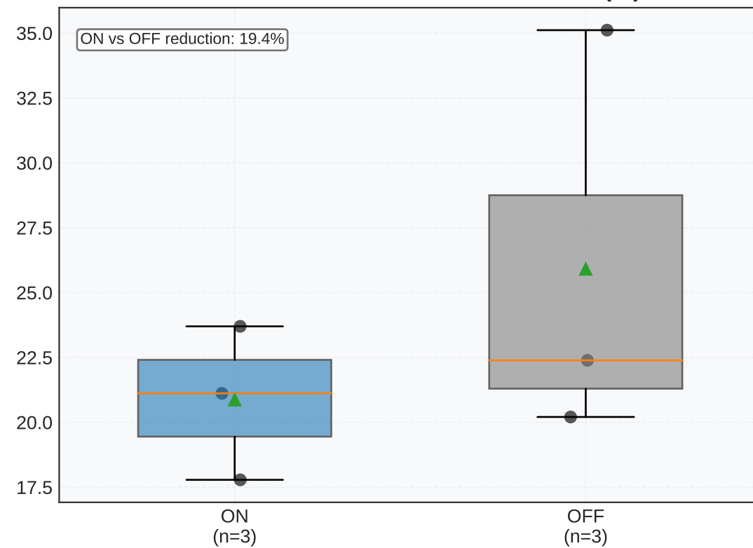
Attack window mean controller CPU (%)
