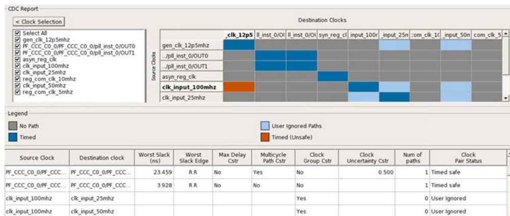
Figure 8-13. CDC Table in Sync with Clock Selection Section
