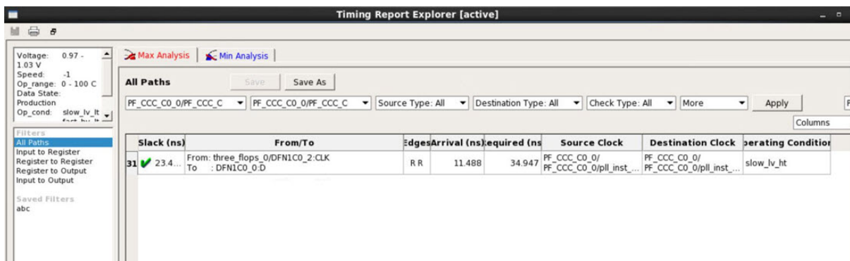
Figure 8-17. Timing Report Explorer
