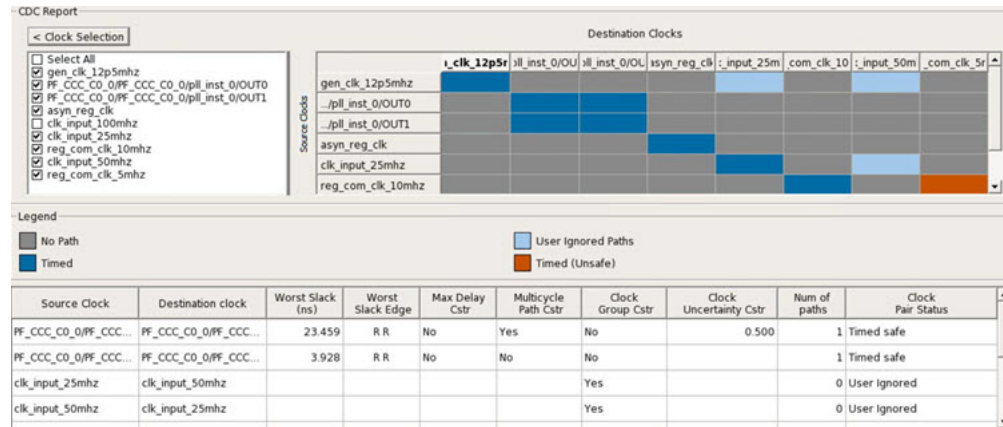
Figure 8-14. Deselecting a Clock in Clock Selection Section Syncs the Path Table Accordingly
