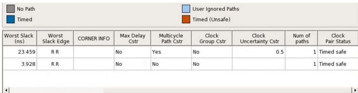
Figure 8-15. CDC Report When Timed Button is Selected in CDC Category
