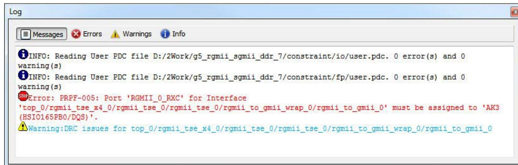
Figure 10-2. Log Window
