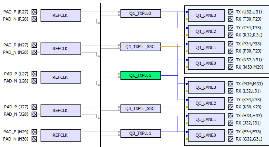
Figure 7-15. Q1_TXPLL1 to Four Lanes Connection (Before Placement)
