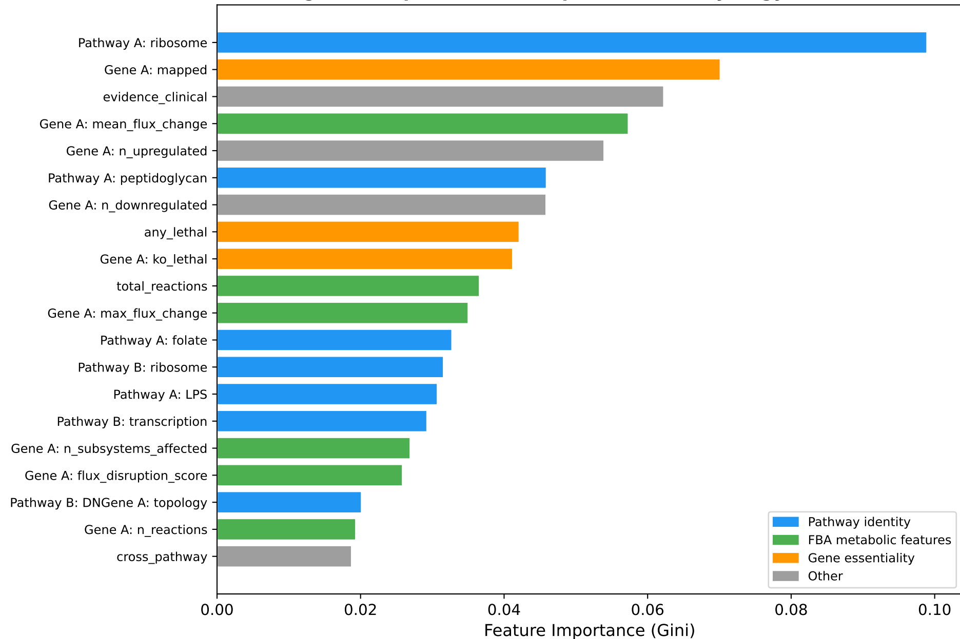
Figure 4. Top 20 Feature Importances for Synergy Prediction
