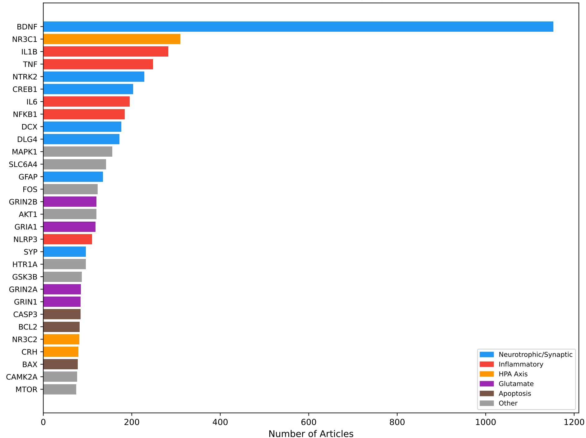
Figure 2. Top 30 Genes in Chronic Stress × Brain Literature (N = 9,585 articles, 2,157 unique genes)
