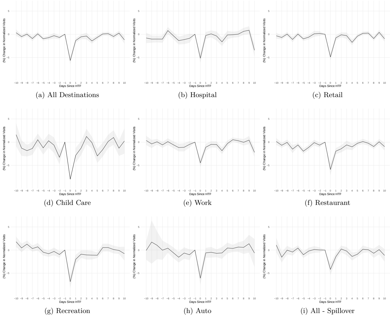
Figure 4.1: The Effects of HTF on the Number of Daily Visits. Panels (a)-(i) show the impact of HTF on the number of visits in 10 leads and lags. Regression models are estimated in levels, and the estimates are divided by the mean of each dependent variable to express in percentage terms. We control for county by year, zip code by month, and day-of-week fixed effects. Grey areas show the 95% confidence interval.
