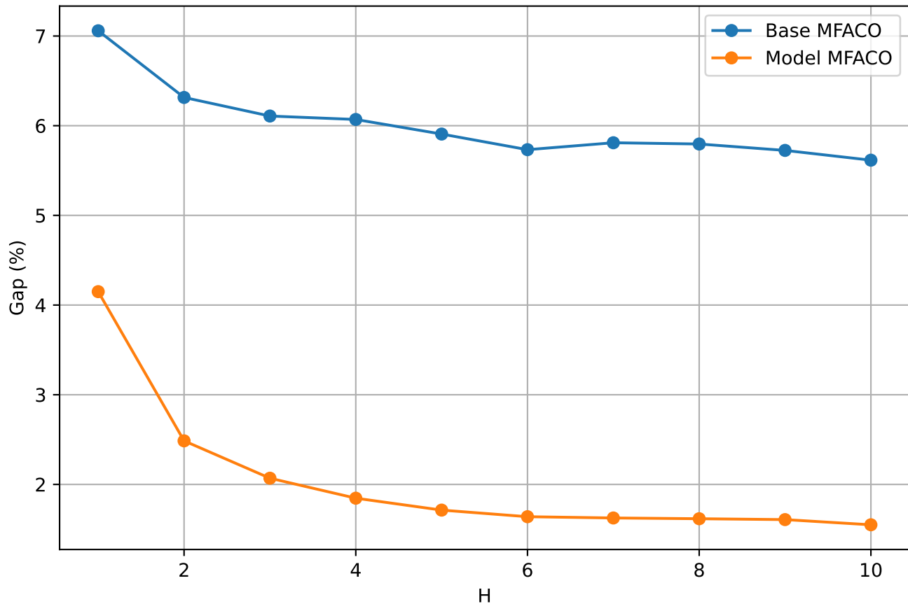
Gap (%) vs H Steps
