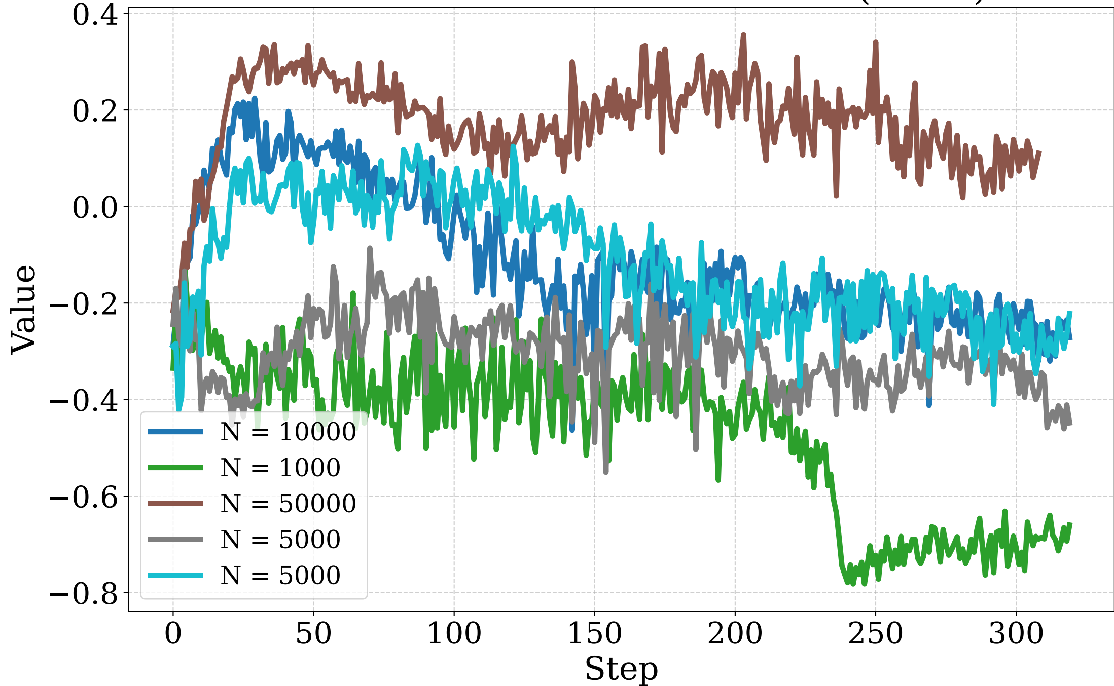
Model vs. Pheromone Correlation (CVRP).
