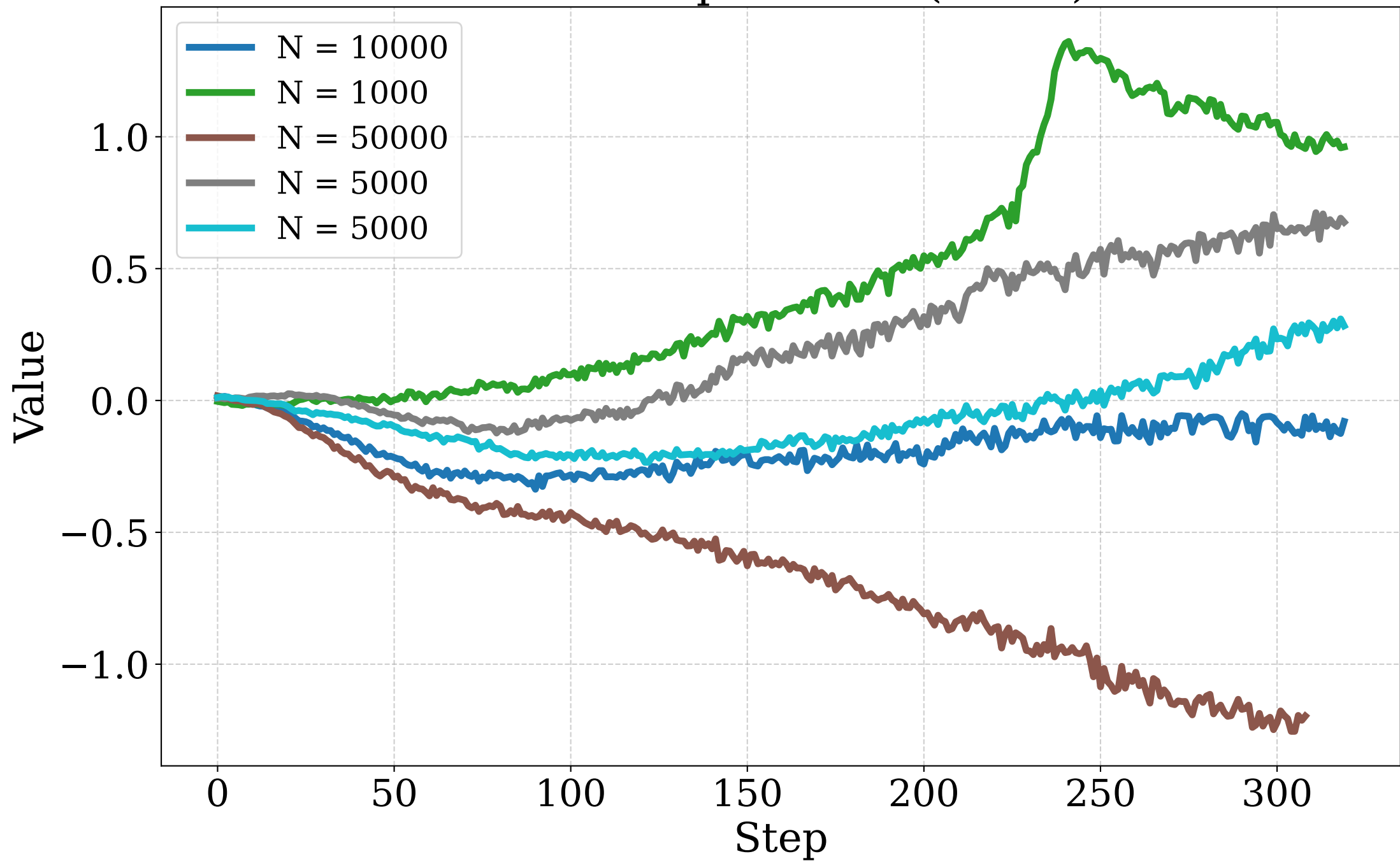
Model Output Mean (CVRP).
