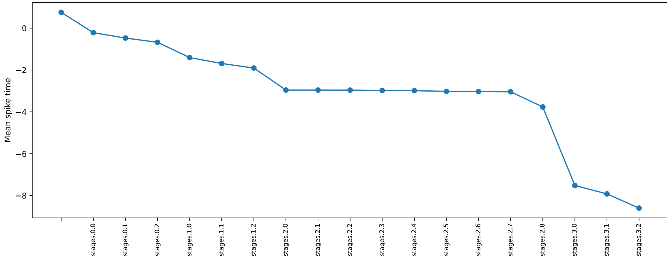
Mean spike time per layer (corrected)
