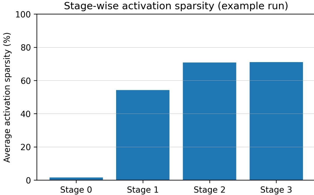
Figure 5. Example stage-wise activation sparsity (Try 3-B snapshot). Early stages exhibit low sparsity compared to later stages, highlighting opportunities to further sparsify early feature extraction.
