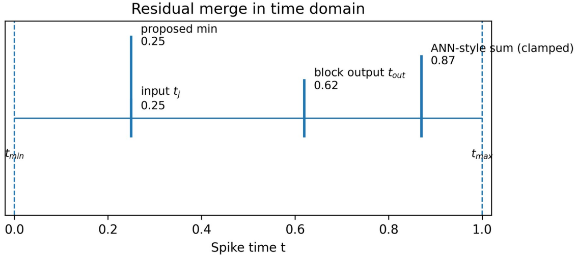
Figure 3. Illustration of residual merging in the time domain. ANN-style summation delays spike times, while the proposed minimum merge preserves the earliest (most salient) spike.
