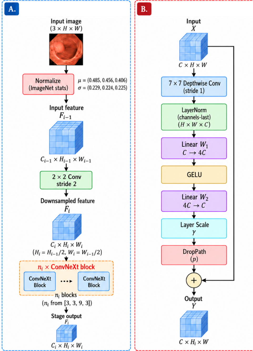
Figure 2: ConvNeXt-Tiny encoder structure. (A) Stage-level processing after the one-time ImageNet normalization: Stage 1 uses a 4 \times 4 stride-4 stem, while subsequent stages use 2 \times 2 stride-2 downsampling and repeat ConvNeXt blocks according to depths [3, 3, 9, 3] . (B) An individual ConvNeXt block, comprising a 7 \times 7 stride-1 depthwise convolution, channels-last Layer Normalization, linear expansion from C to 4C , GELU, linear projection from 4C to C , layer scaling, DropPath, and residual addition.
