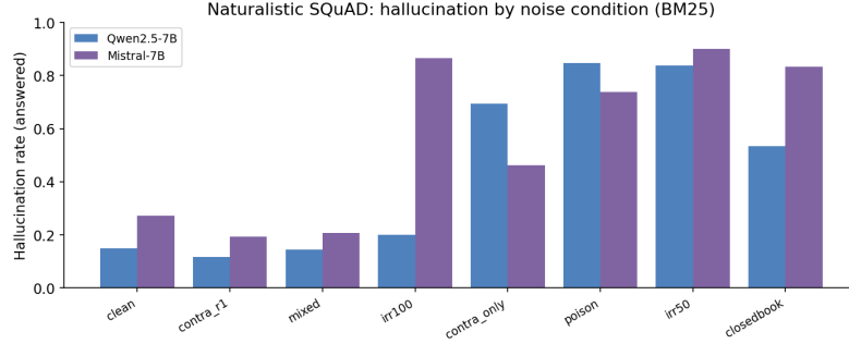
Fig. 7 Per-condition hallucination rate under real SQuAD retrieval. Closed-book and missing-evidence conditions and PoisonedRAG poisoning drive the highest hallucination; the clean condition already sits at 0.15 to 0.28, which sets the realistic selective-risk target at \alpha = 0.20 .
