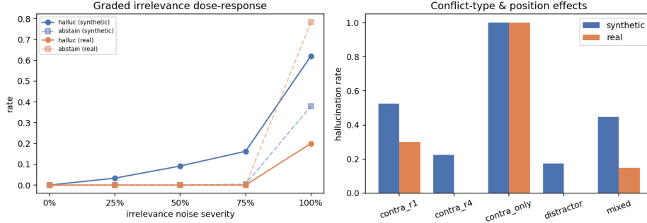
Fig. 2 Left: graded irrelevance dose-response. Hallucination rises smoothly with severity; abstention appears only at total irrelevance, and reliably only in the parametric-knowledge regime. Right: conflict-type and position effects.
