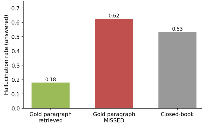
Fig. 9 Purely natural retrieval noise on the full SQuAD pool with no injection. Hallucination rises from 0.179 when the gold paragraph is retrieved to 0.625 when the retriever misses it, with closed-book at 0.533.
