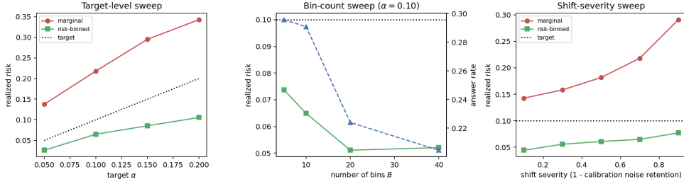
Fig. 4 Sensitivity of the guarantee. Left: target-level sweep; marginal CRC scales its violation with \alpha while risk-binned certification tracks below target. Centre: bin-count sweep at \alpha = 0.10 ; five bins are too coarse, ten suffice. Right: shift-severity sweep; marginal risk grows monotonically from 0.143 to 0.291 as calibration sees less noise, while risk-binned certification stays controlled throughout.
