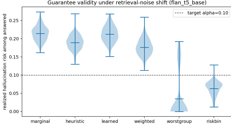
Fig. 3 Realized risk among answered queries across 200 resplits at \alpha = 0.10 (dotted line). The four standard methods lie entirely above the target; risk-binned certification is the only practical method below it.
