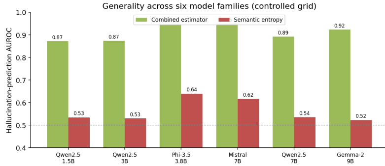
Fig. 6 Combined risk estimator versus the sampling-based semantic entropy baseline across the six instruction-tuned families of Table 6. The combined estimator (AUROC 0.87 to 0.95) separates cleanly from semantic entropy (0.52 to 0.64) on every family, and the gap does not shrink with model scale.
