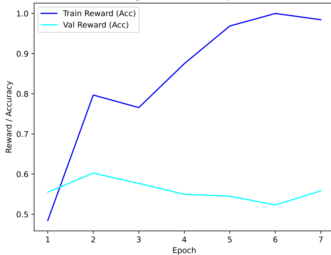
RL Agent Reward over Epochs
