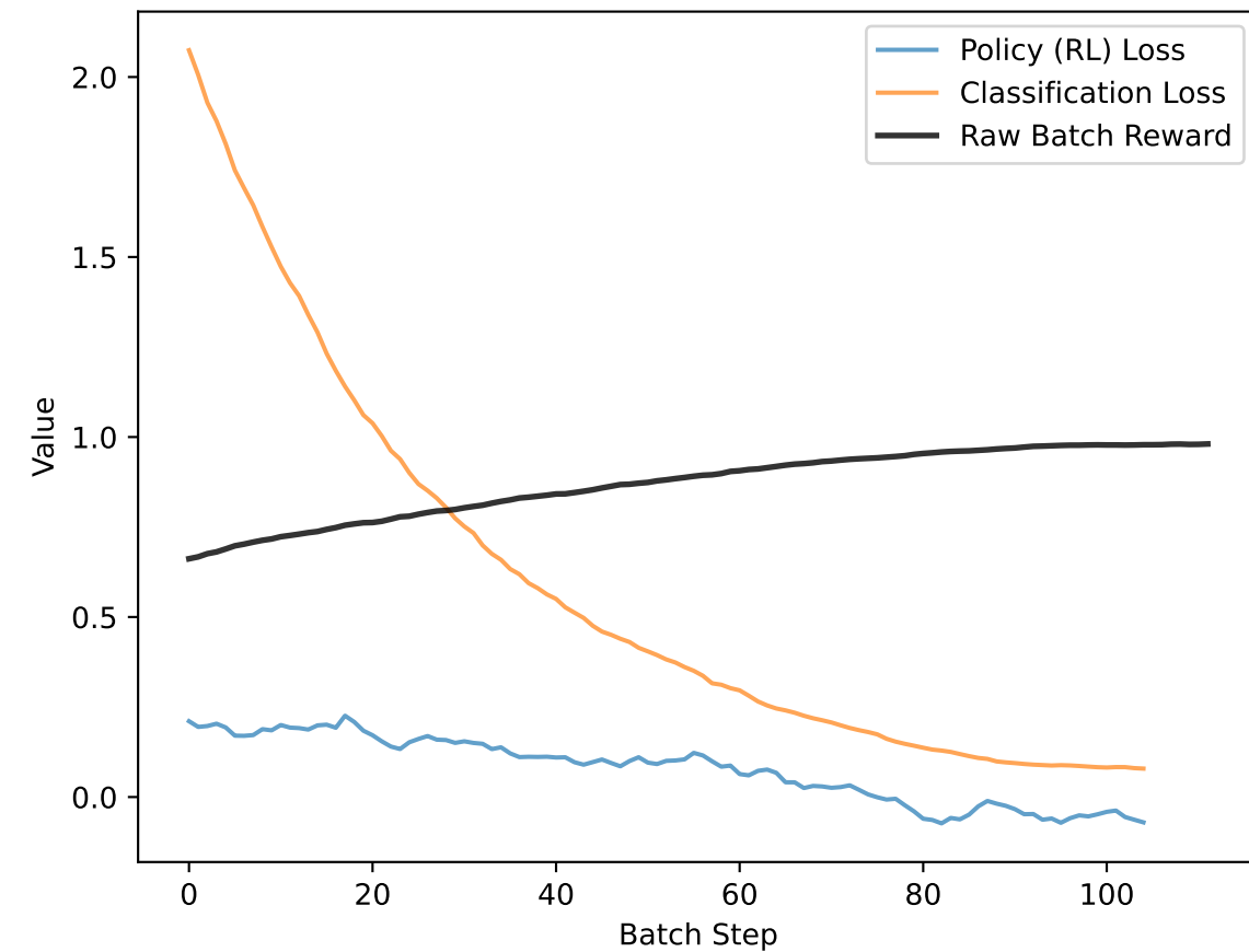
RL Internal Metrics (Smoothed)
