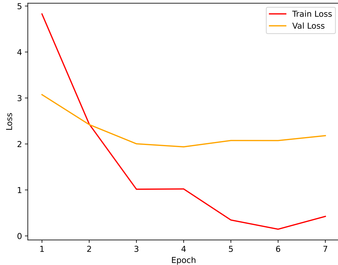
Total Loss (Train vs Val)
