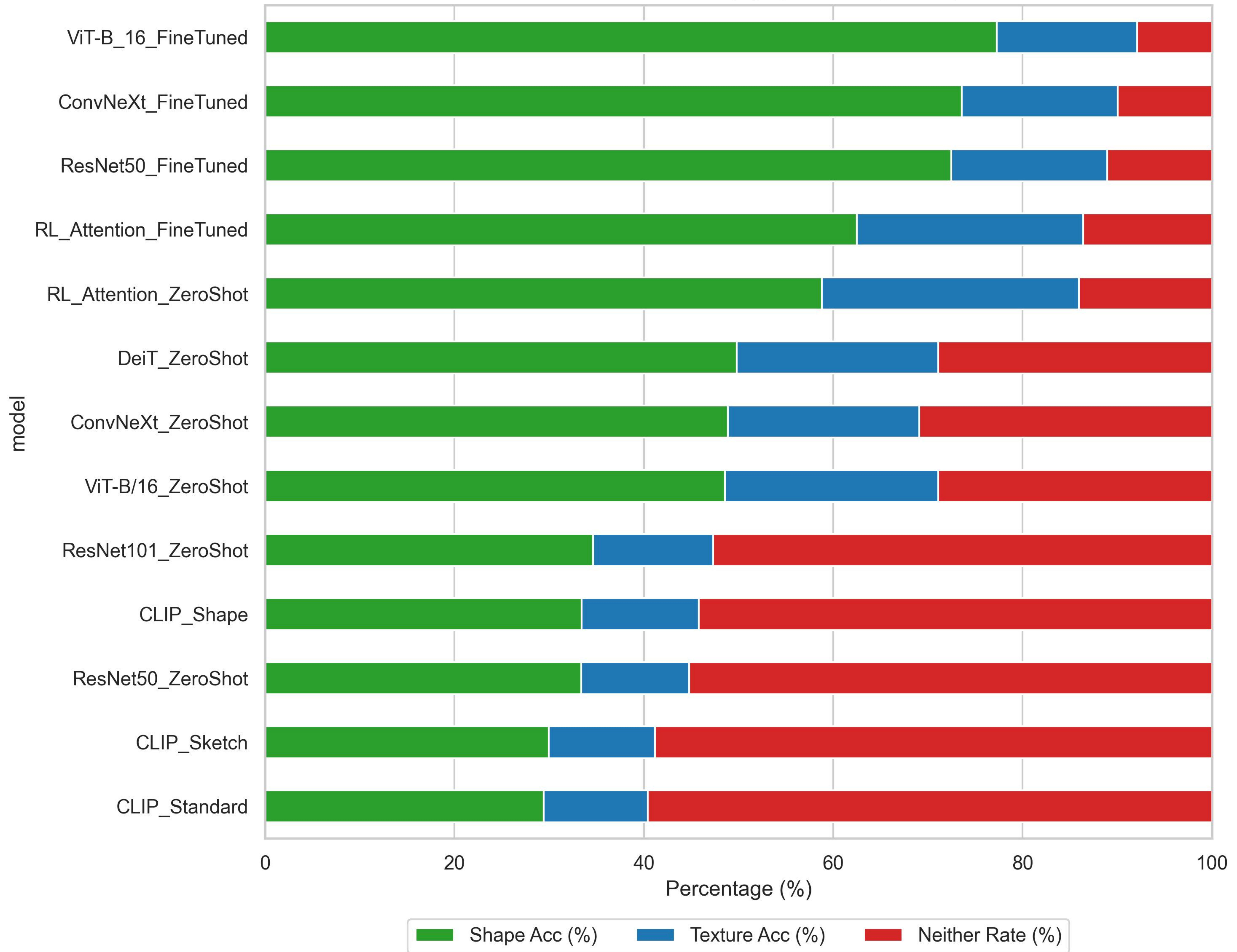
Absolute Cue Sensitivity (Triple Decomposition)
