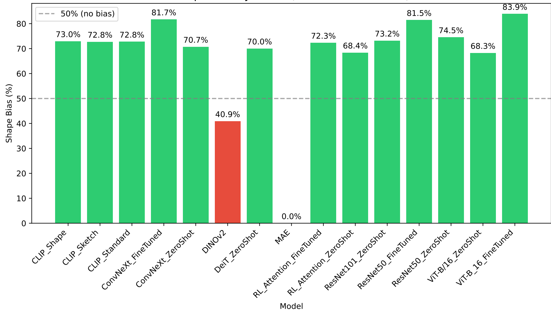
Shape Bias by Model (Geirhos et al. Metric)
