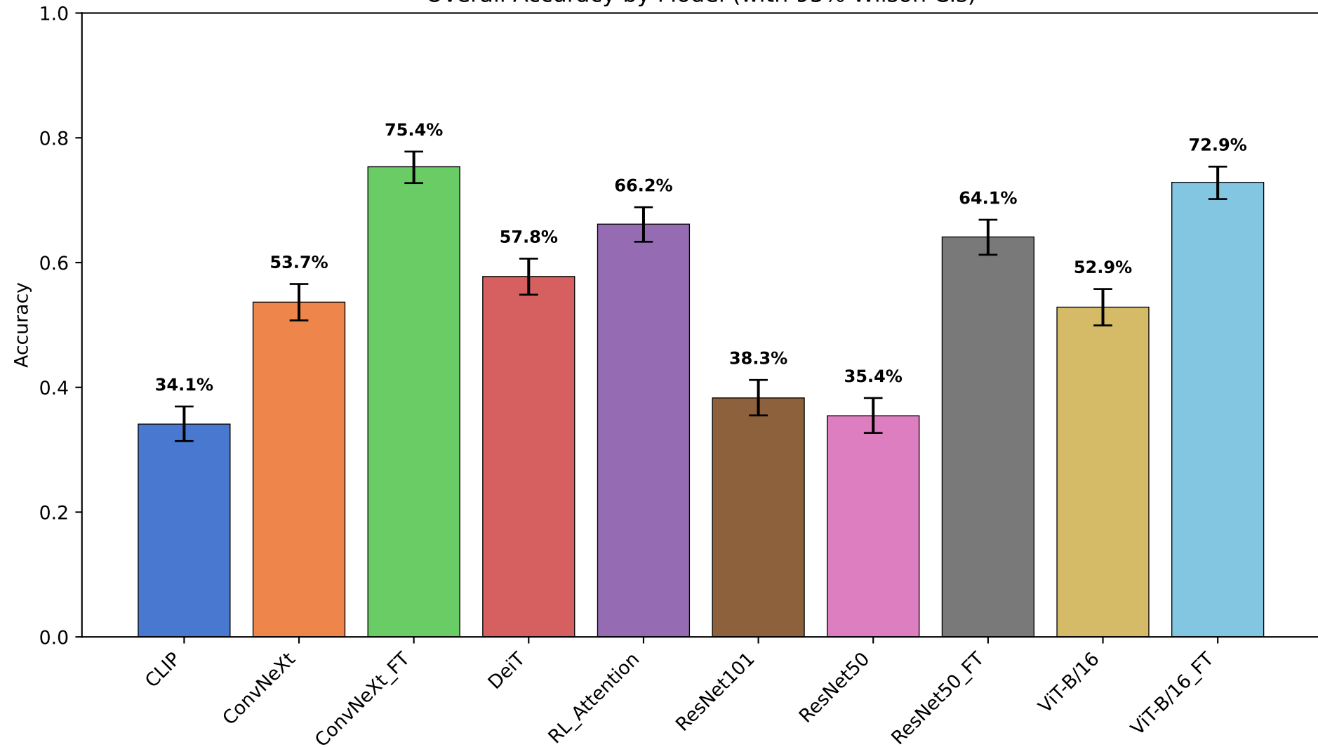
Overall Accuracy by Model (with 95% Wilson CIs)
