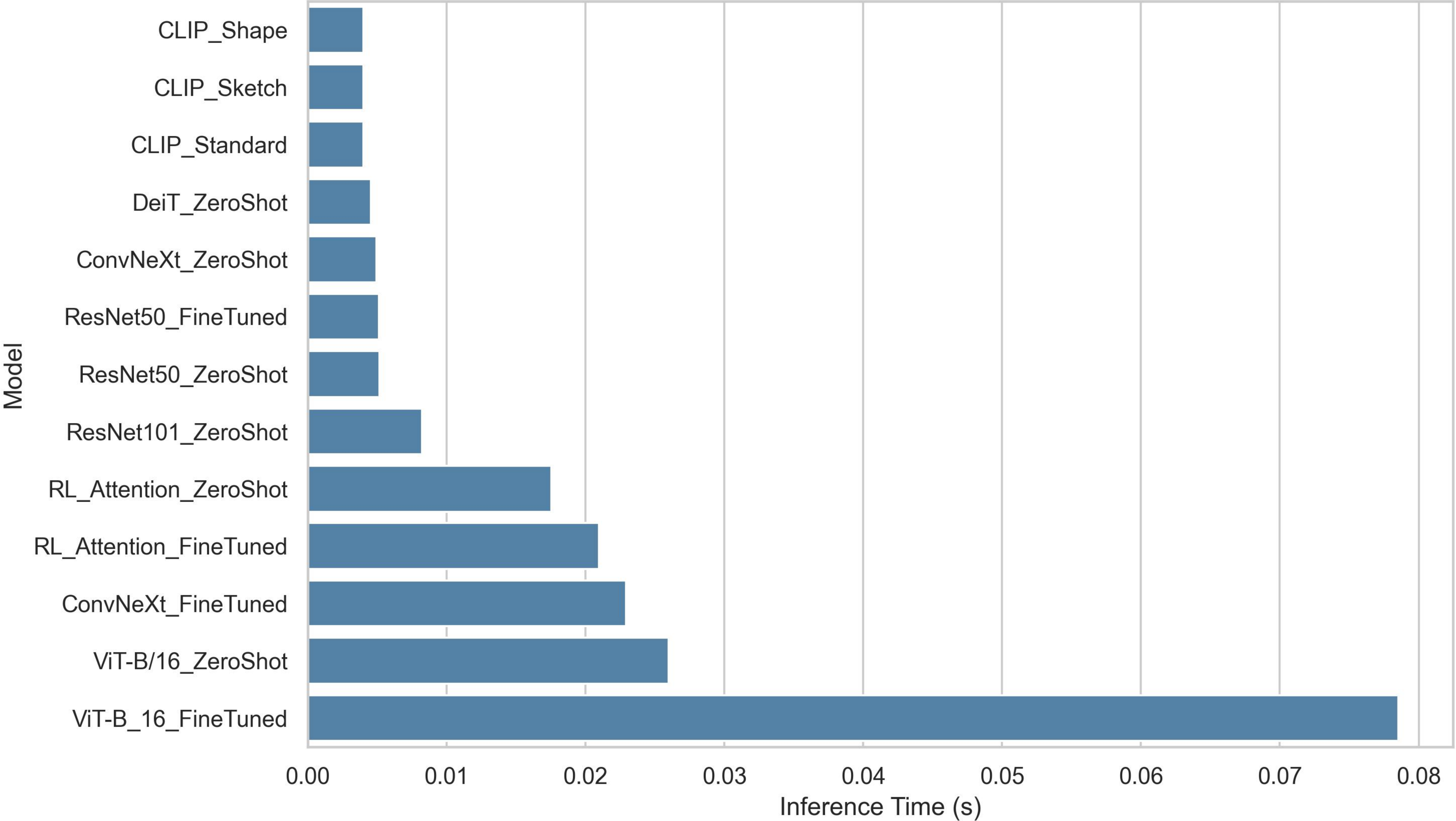
Average Inference Time per Image (Seconds)
