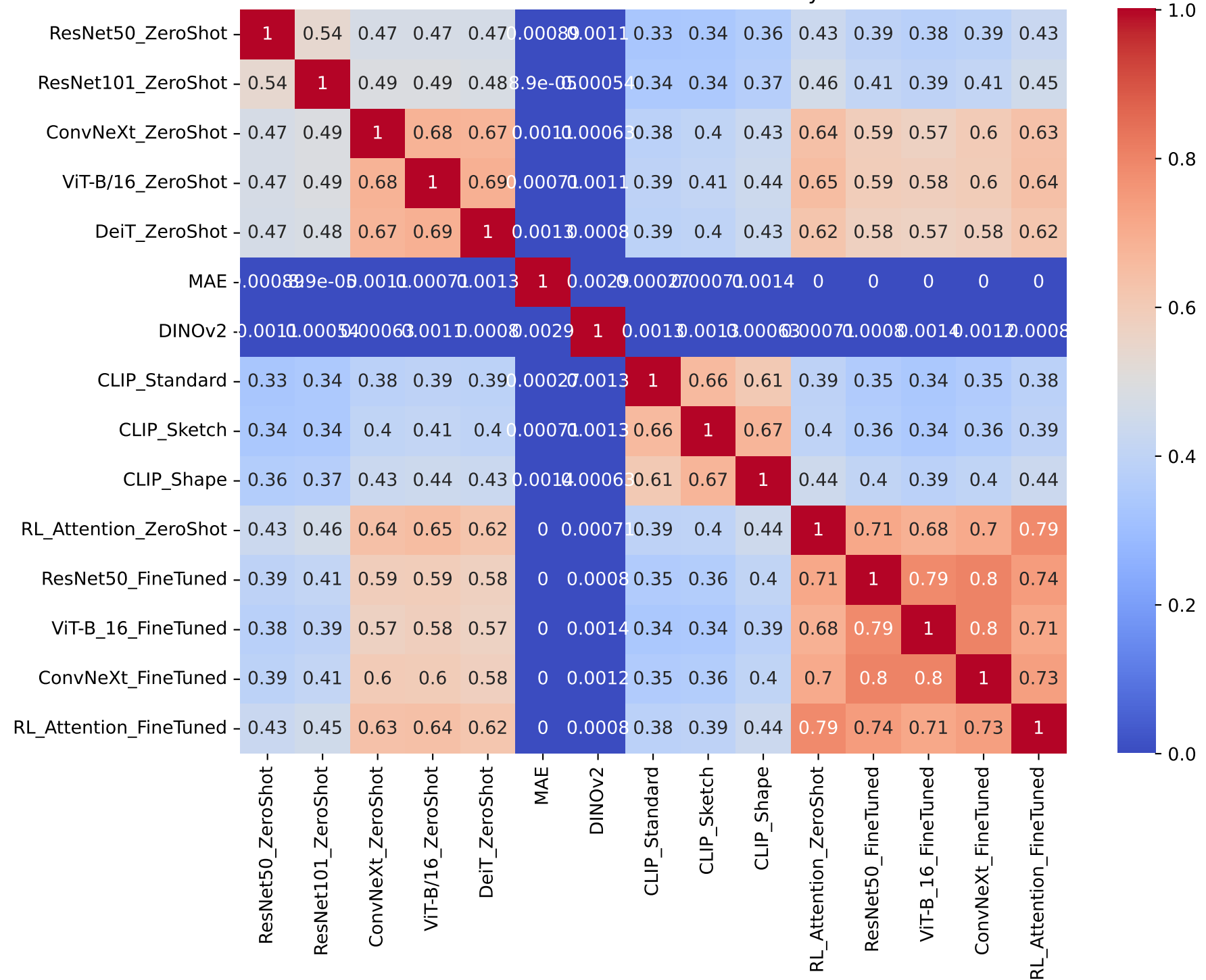
Model-Model Error Consistency
