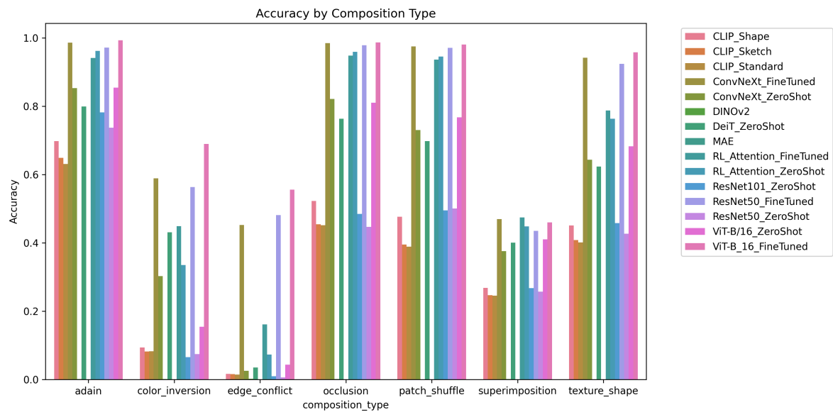
Figure 3: Breakdown of accuracy metrics grouped by composition type.
