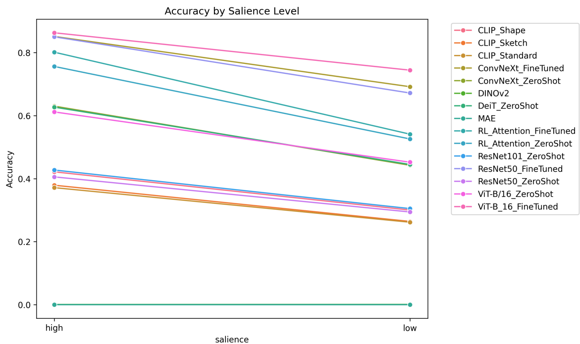
Figure 4: Performance degradation when moving from high to low shape saliency.
