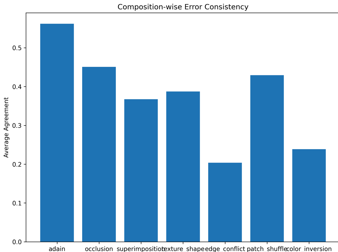
Figure 6: Consistency clustered by composition method.
