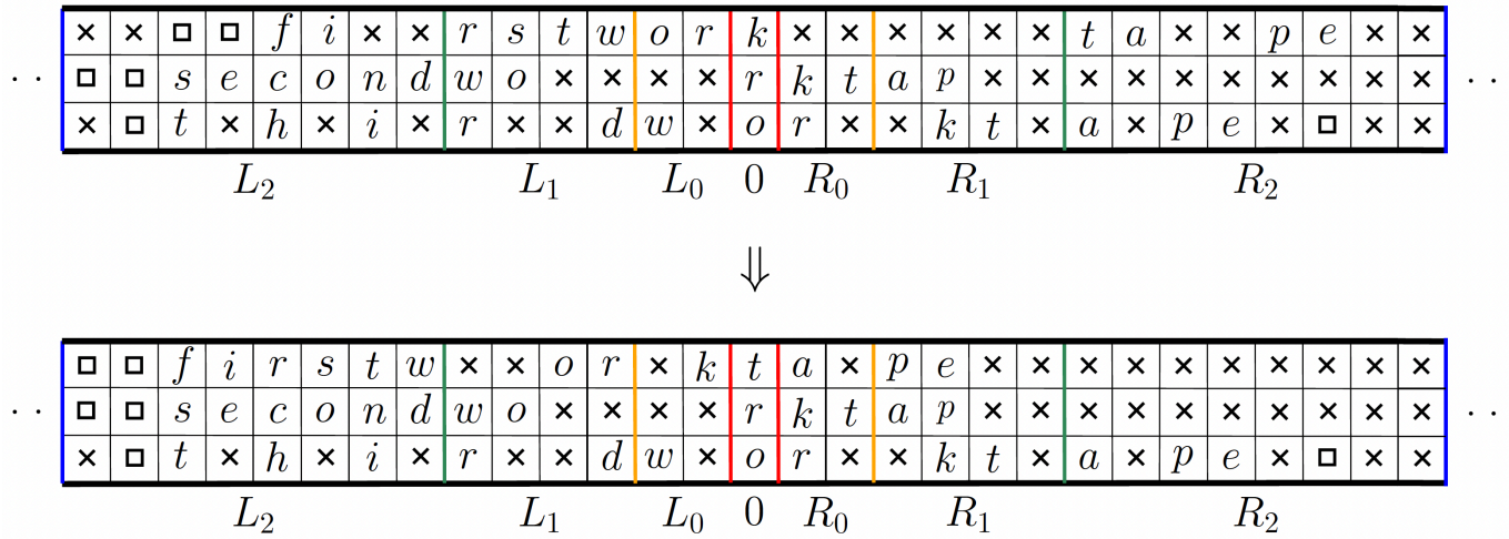
Figure 1: 证明图
