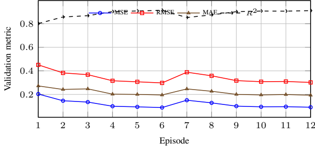
Fig. 4. Recorded validation metrics across the 12 warm-start episodes.
