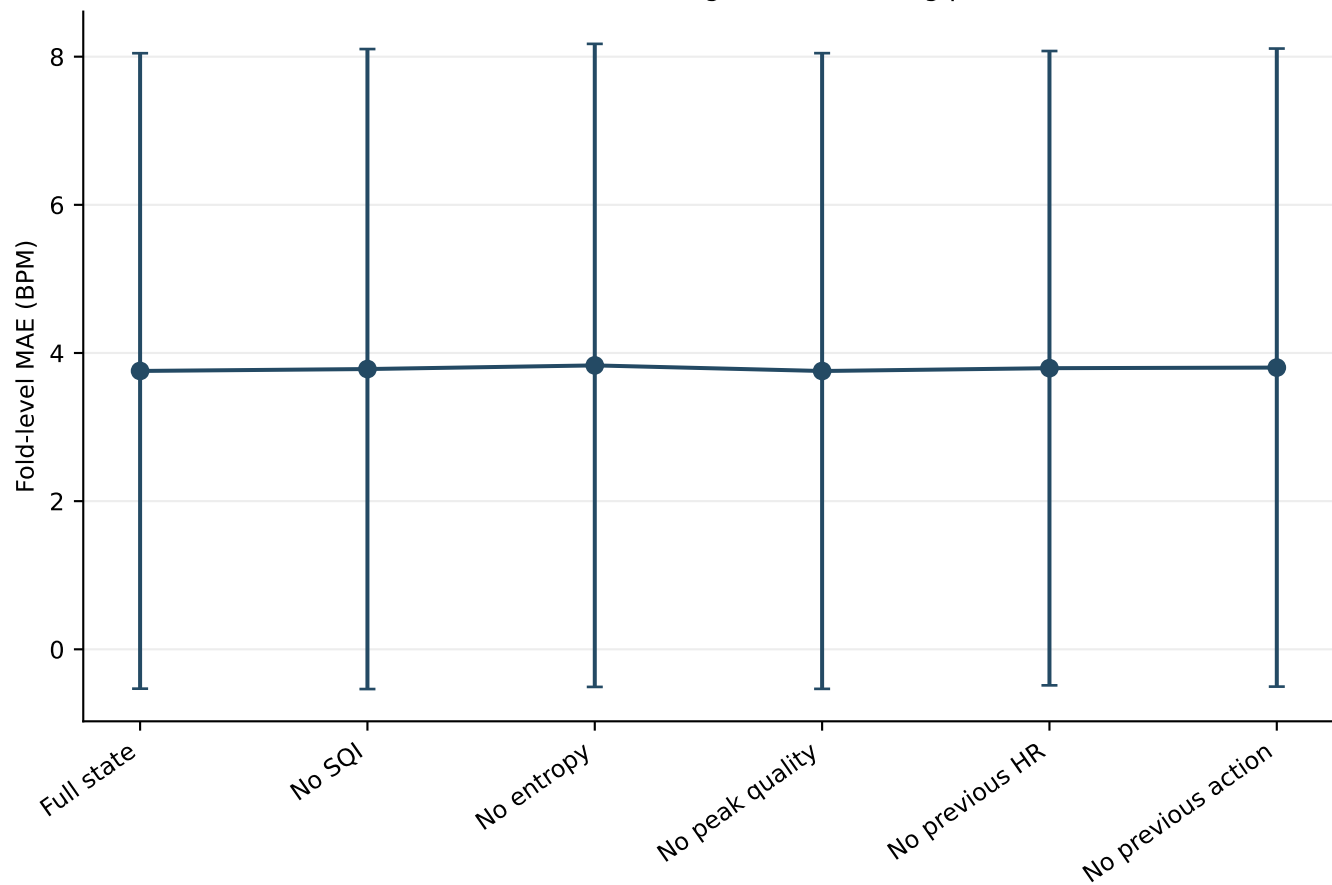
State ablation: Q-learning with 25 training passes
