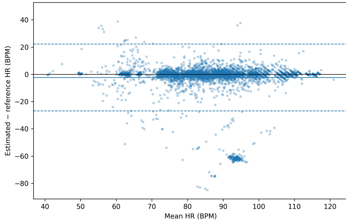
Q-learning
