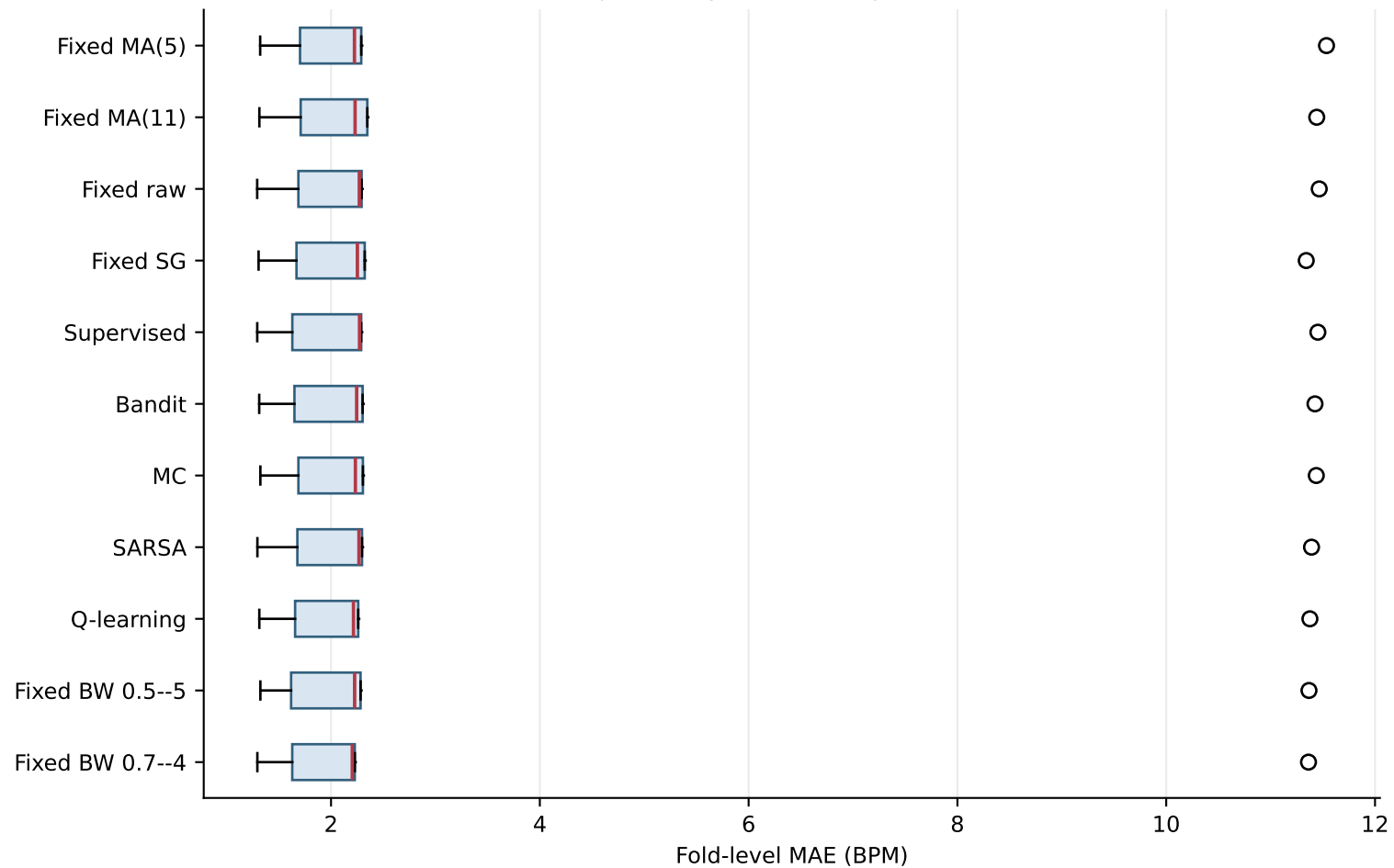
Subject-independent fold performance
