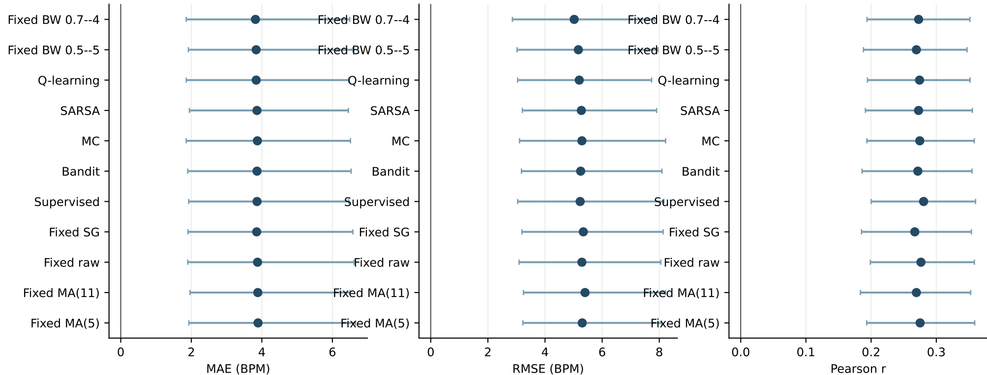
Subject-level means with 95% bootstrap CIs
