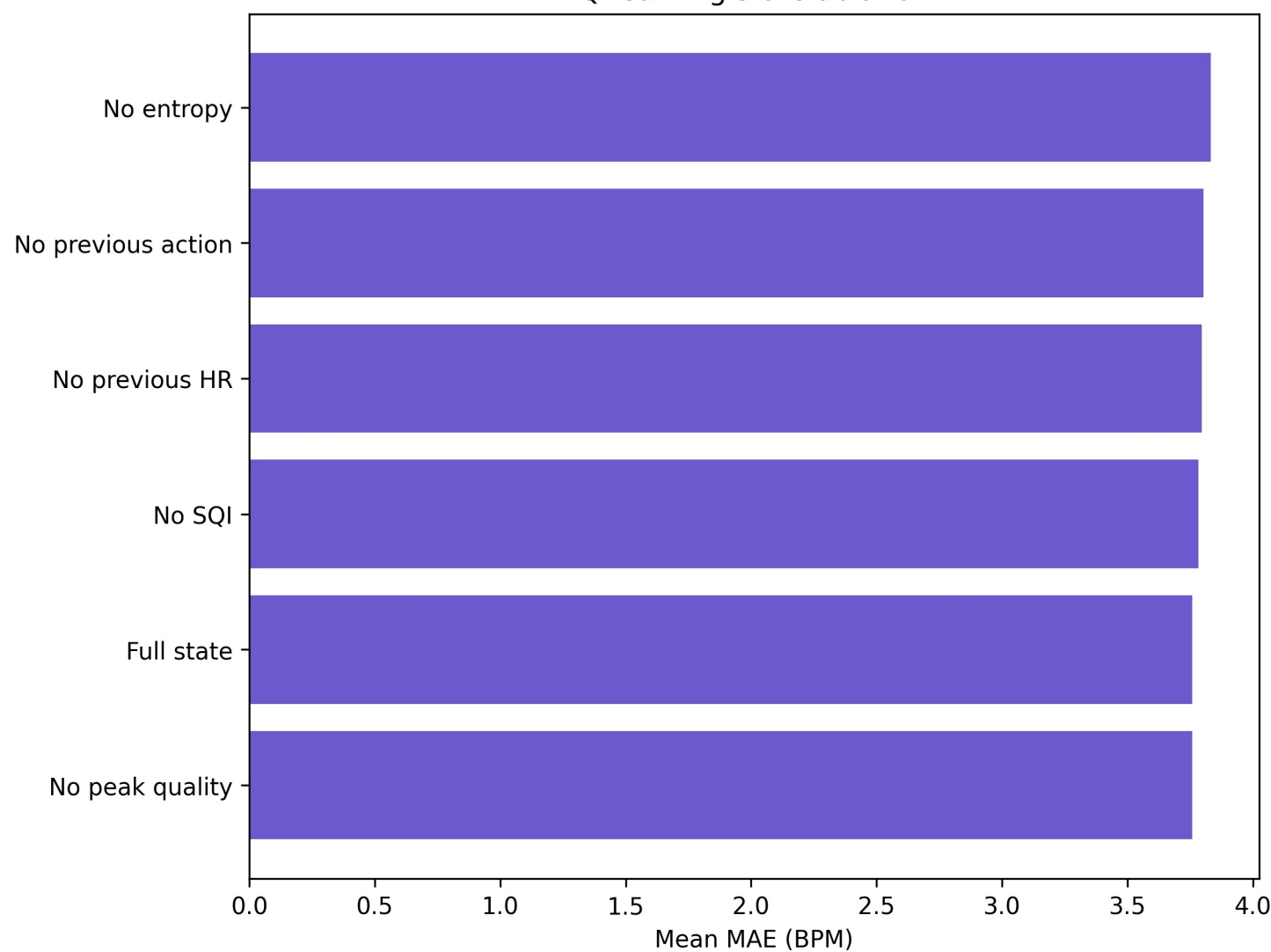
Q-learning state ablation
