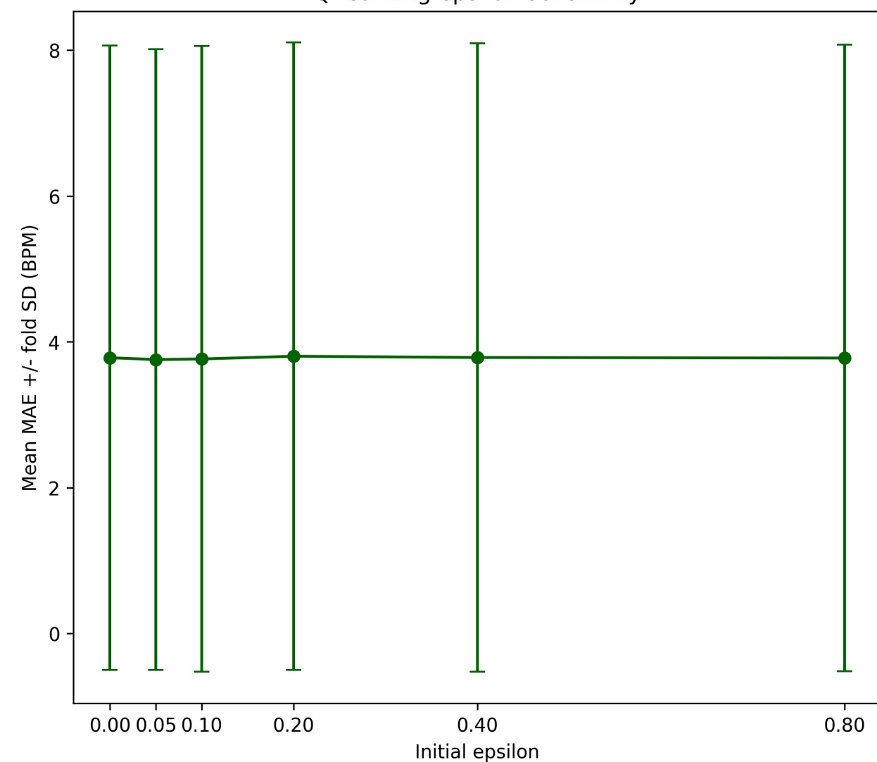
Q-learning epsilon sensitivity
