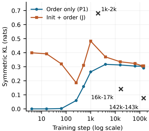
A Functional divergence
