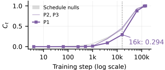
C Raw endpoint-direction alignment
