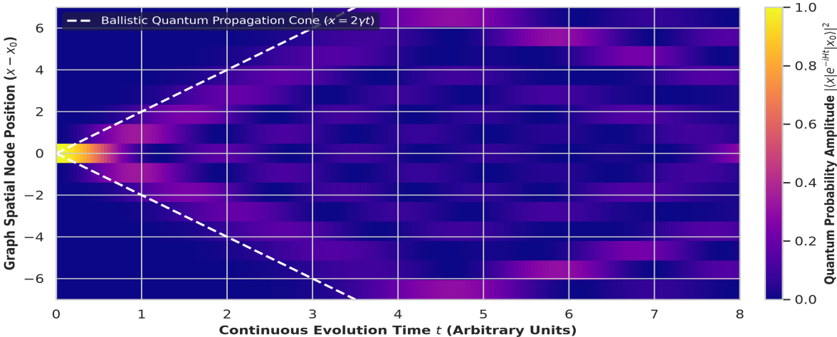
Figure 4: Continuous Time-Evolution & Ballistic Light-Cone Propagation
