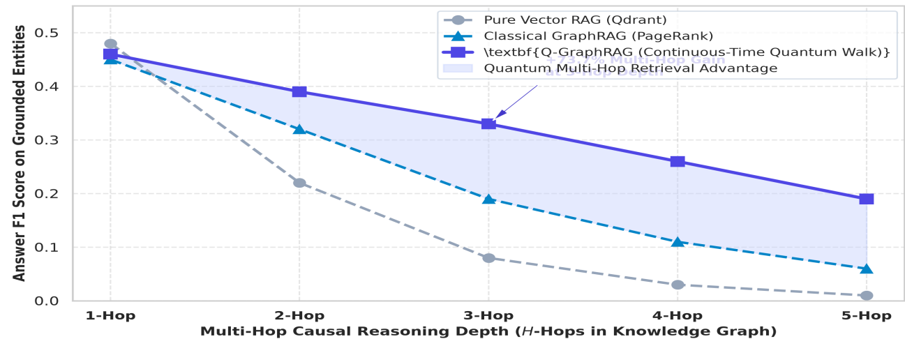
Figure 7: Answer F1 robustness as a function of graph depth H. While classical vector search degrades rapidly at H \geq 2 and classical PageRank suffers from hub diffusion, Q-GraphRAG achieves a +73.7% Answer F1 advantage at H = 3 hops.
