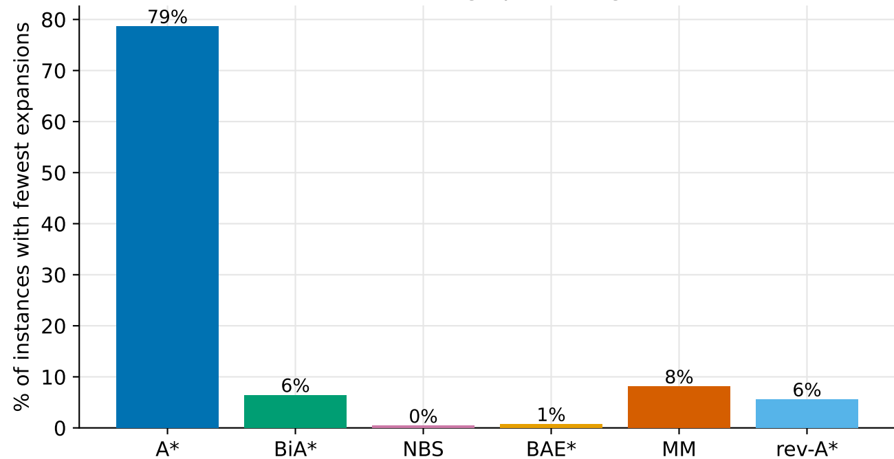
Per-instance winner among optimal algorithms (n=947)
