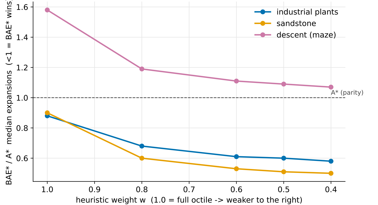
Heuristic-strength crossover: BAE* increasingly beats A* as the heuristic weakens
