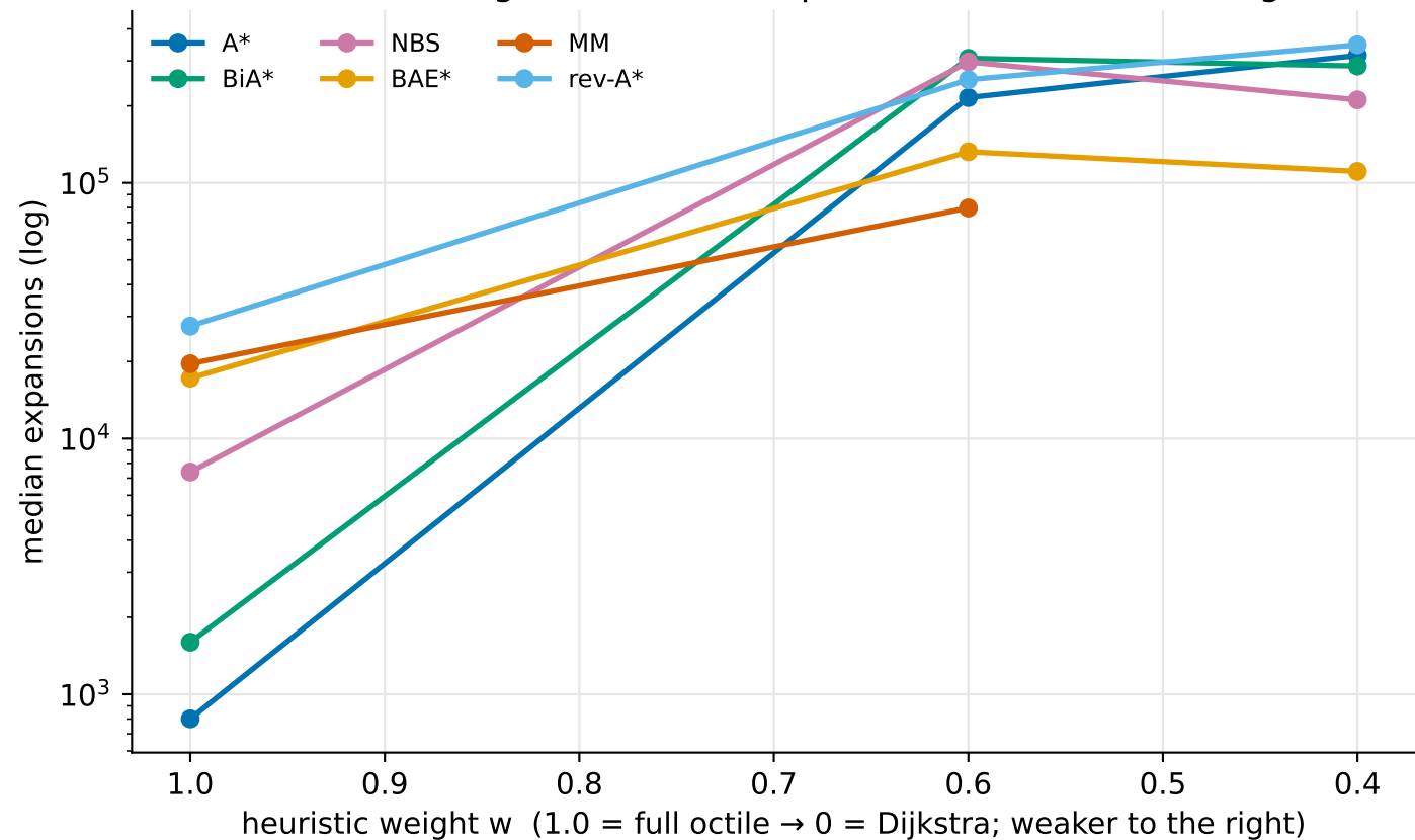
Heuristic-strength crossover: expansions vs. heuristic weight
