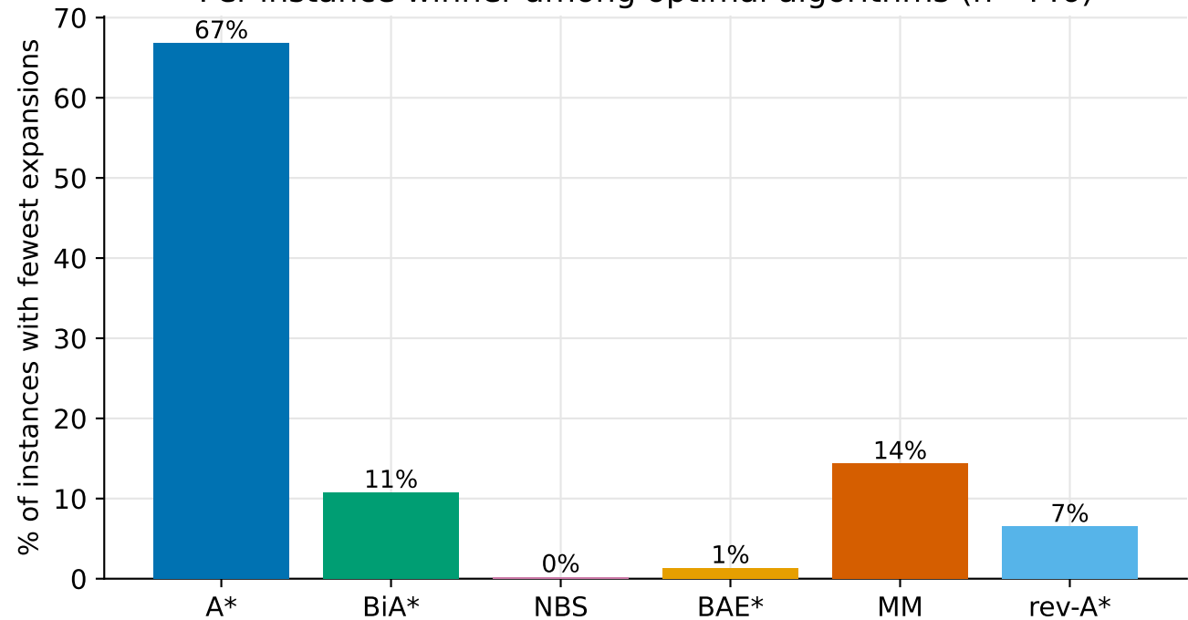
Per-instance winner among optimal algorithms (n=446)
