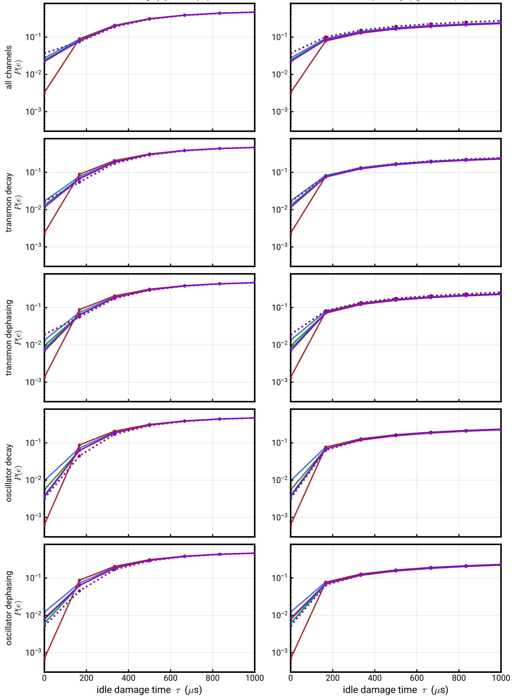
oscillator decay ( T_1 = 1000 \mu\text{s} )
