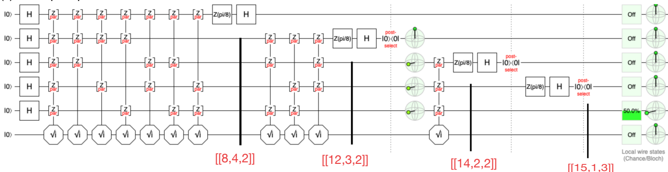
(b) [[8,4,2]]: CCZ-to-T
