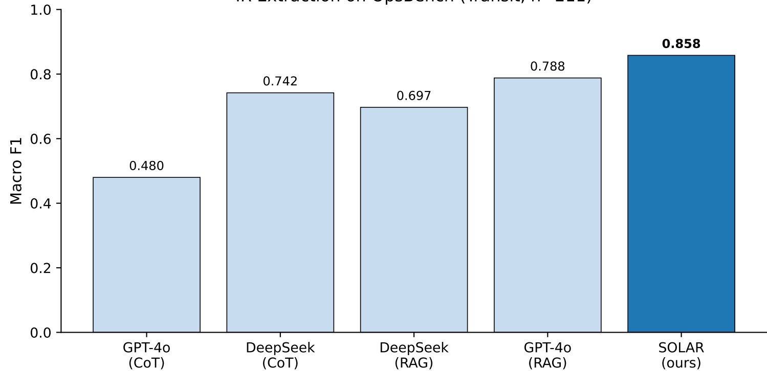
IR Extraction on OpsBench (Transit, n=211)
