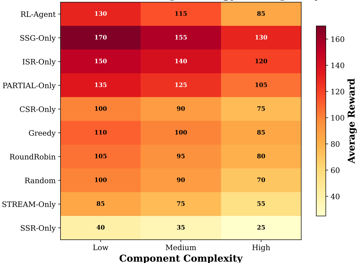
Performance Heatmap: Strategy × Complexity
