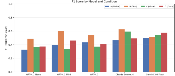
Figure 3: F1 score by model and condition.
