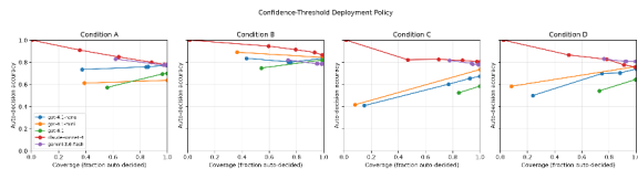
Figure 8: Confidence-threshold deployment policy,
