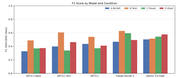
Figure 3: F1 score by model and condition.
